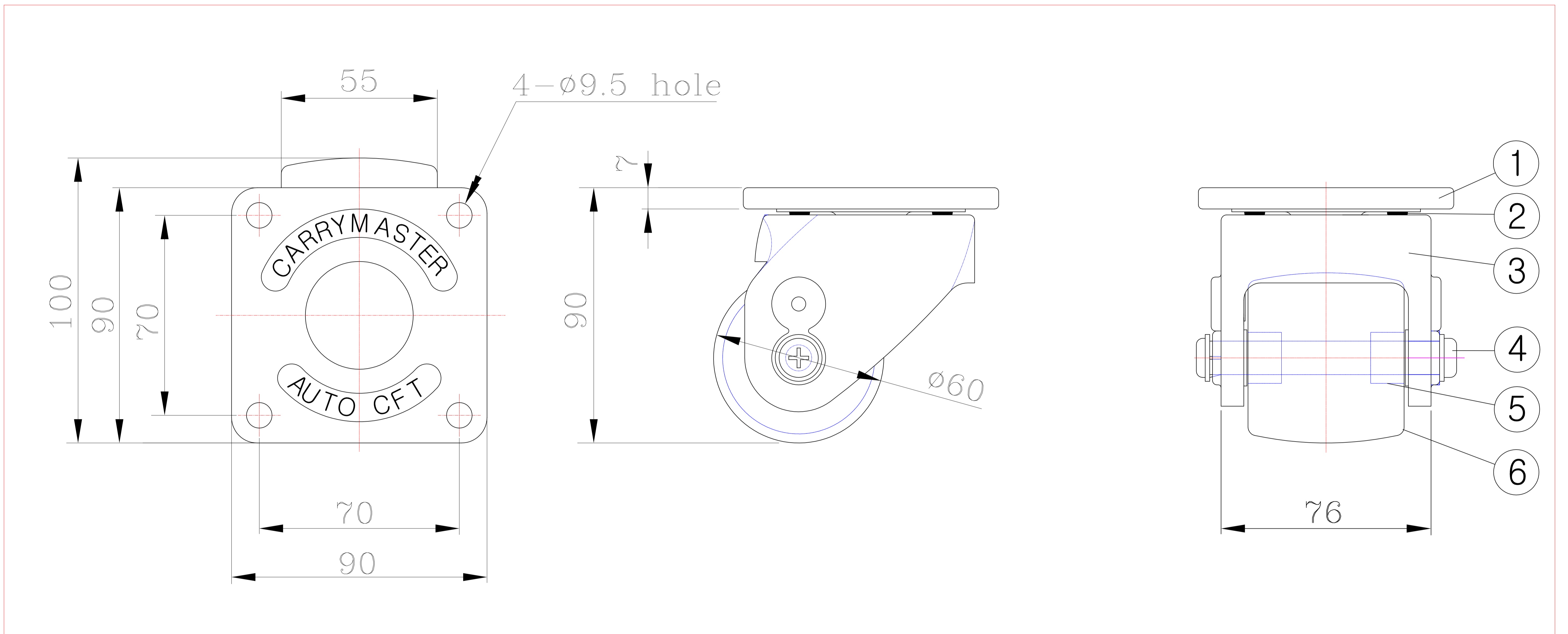
ACM-600FU TYPE
